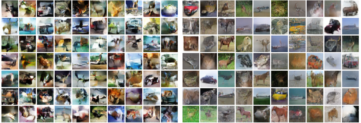
Figure 21: Samples on CIFAR-10. Left: Decoded samples drawn from the prior of the autoencoder: x = G(z) , z \sim \mathcal{N}(0, \mathbf{1}) . Right: Decoded samples drawn from the prior of the transformer: x = G(T^{-1}(\tilde{z})) , \tilde{z} \sim \mathcal{N}(0, \mathbf{1}) .
